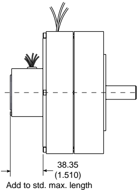
Dimensions in mm (inches). Product designed in inches. Metric conversions provided for reference only.
