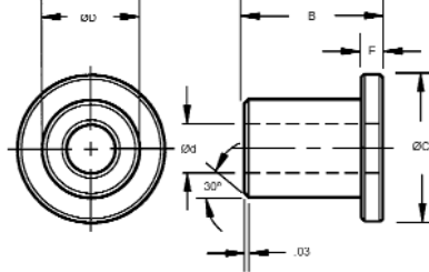
Flanged
