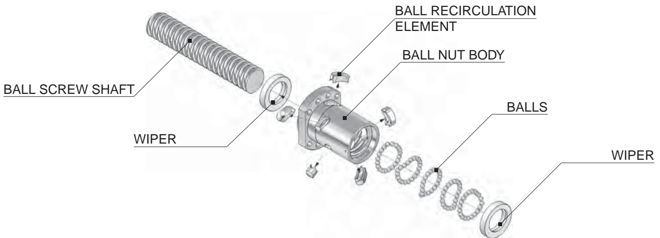
Fig. 1 - Ball screw assembly
