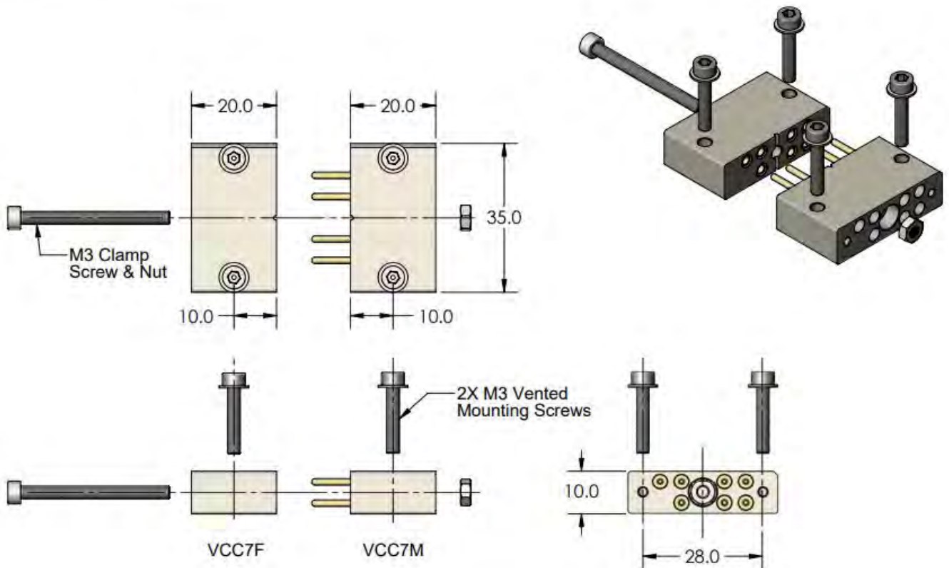
VCC7 - In-Vacuum Connectors
