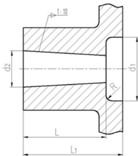
Z Type:Long Taper Bore with Counterbore
