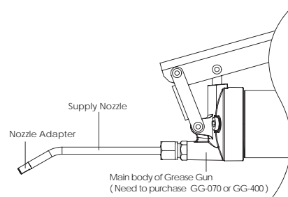
Greasing Diagram
