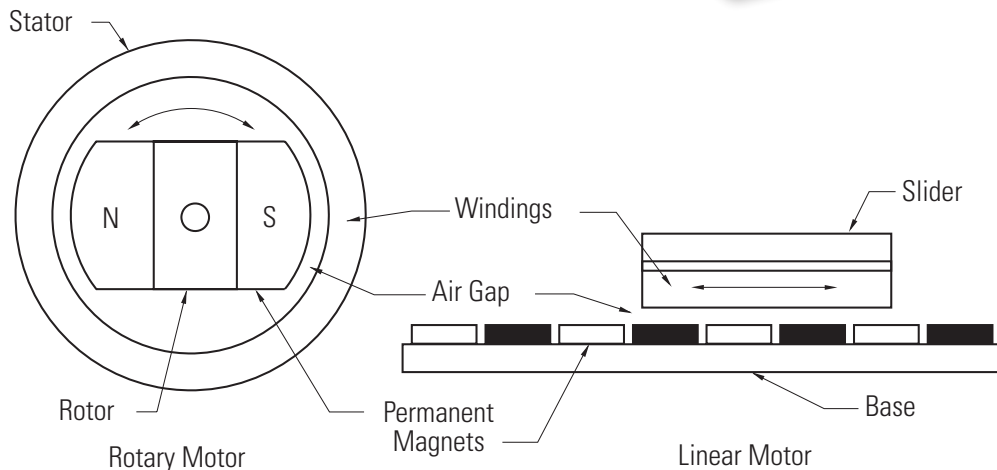
Rotary Motor Rolled Out Flat
