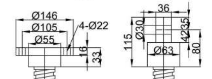
I Top Plate II Clevis End
