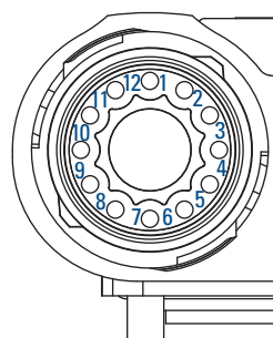
Resolver Connector
