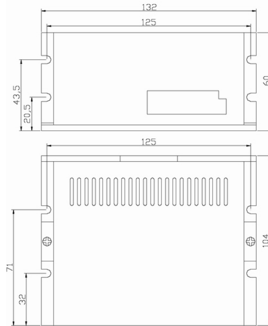
Figure 1: Mechanical specifications
